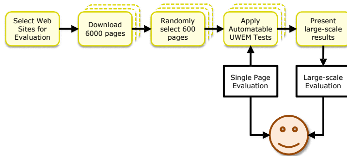
Fig. 1. EIAO Workflow
